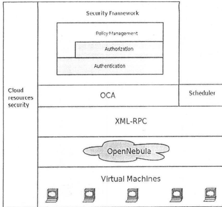
Figure 3.4 Architecture of Cloud Security Framework
