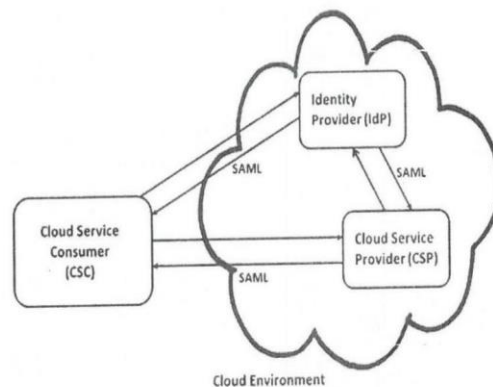
Figure 3.1 Architecture of Access Control Model for Cloud
