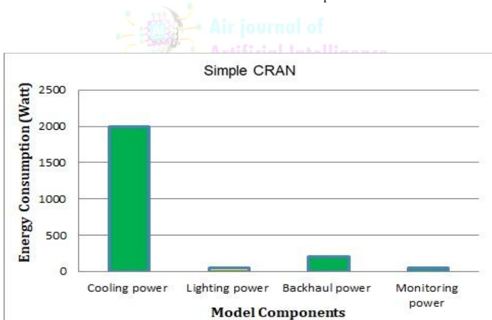
Fig. 4. Simple C-RAN energy consumption.
