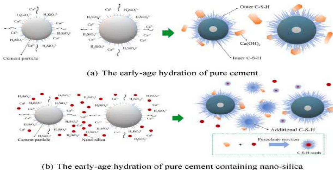
(b) The early-age hydration of pure cement containing nano-silica Image 1: Effect of nano-silica on mechanical, microstructural and durability properties of cement-based
